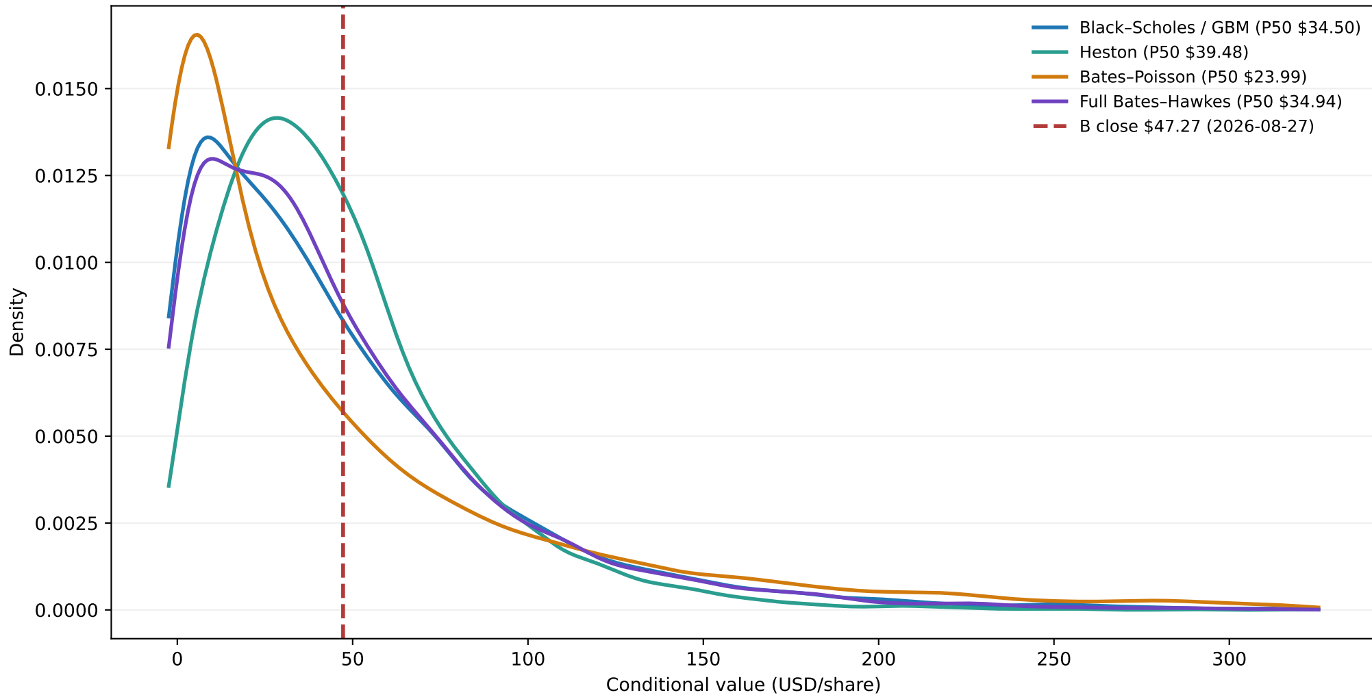
Barrick conditional value distributions by gold-price model
